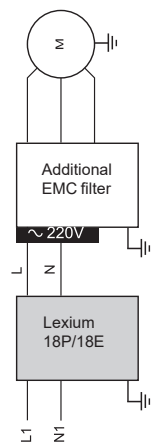
Lexium 18P/18E servo drive with additional EMC filter
