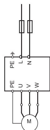
LXM18P/18E servo drive, BCH18 servo motor with fuse protection
